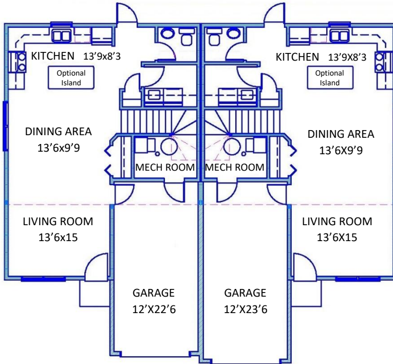
MAIN FLOOR
